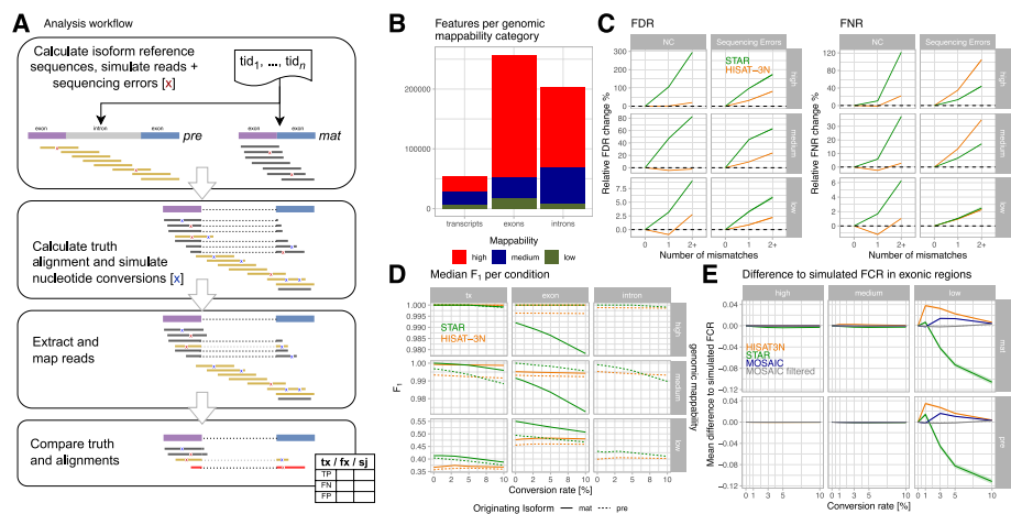
Fig. 1 Analysis workflow and NC mapping accuracies for simulated mouse metabolic labeling data. A Analysis workflow overview: briefly, we simulated short reads with realistic sequencing error (red X) for premature and mature isoforms, calculated truth alignments, and injected nucleotide conversions with configured conversion rates. Simulated reads were mapped by the evaluated read mappers and resulting alignments were compared to the simulated data. Finally, grouped count tables with true positive (TP), false positive (FP), and false negative (FN) counts per annotation of interest (tx: transcripts, fx: exons + introns, sj: splice junctions) were created and analyzed. B Numbers of analyzed m_big annotations with high (>0.9), medium, and low (<0.2) mean genome mappability. C Changes of false discovery ( FDR = FP / (TP + FP) ) and false negative ( FNR = FN / (TP + FN) ) rates by number of mismatches per read compared to reads without mismatches, stratified by mappability and type of mismatch (either simulated NC or random sequencing errors). The plots show median FDR/FNR and interquartile regions (shaded areas) across three m_big replicates for STAR (green) and HISAT-3N (orange) alignments. This analysis included ~12B reads originating from premature isoforms and their classification (TP, FP, FN) with respect to whole-transcript annotations. D Median F1 measure per mapper and originating isoform (pre: premature, mat: mature) for different genomic annotations (tx: whole transcript, fx: exons + introns, sj: splice junctions), stratified by mappability. E Mean difference to simulated, exonic FCR (fraction of converted reads) per mapper and for a “mosaic” approach where the mapper with the smallest difference to the simulated value was chosen. The mosaic approach reduces differences to simulated values and when removing exons where none of the two mappers showed good results, reconstruction is nearly perfect (“mosaic filtered,” see main text). Note that a corresponding plot for human data is provided in Additional file 1: Figure S6 for comparison
